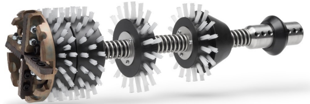
SMART CRUSHER+ 6" & 9" PIPES
